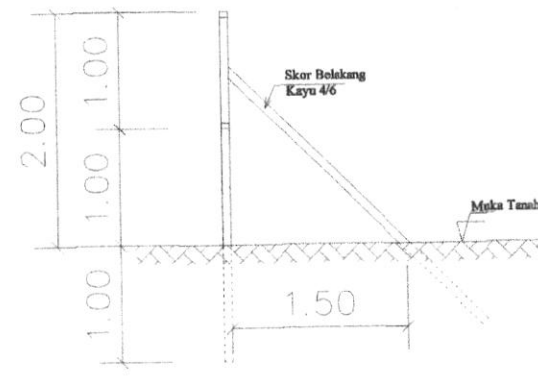
TAMPAK SAMPING →
